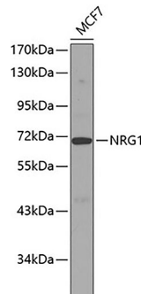
Fig. 1. Western blot analysis of extracts of MCF-7 cells, using NRG1 antibody at 1:10000 dilution. Lysates/proteins: 25µg per lane. Blocking buffer: QuickBlock™ Blocking Buffer (P0231).
